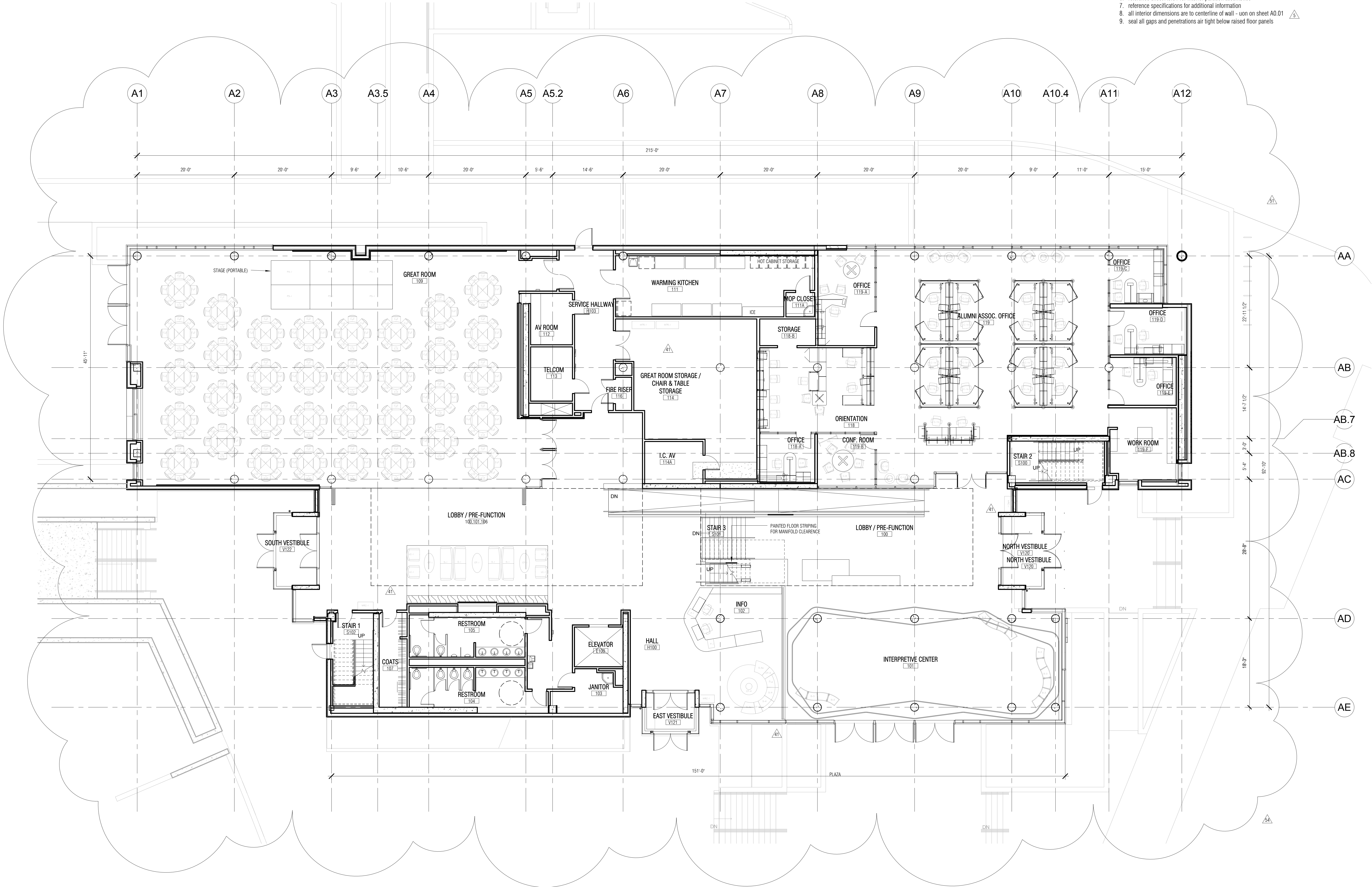
1 LEVEL 01 Furniture Plan A1.51 1/8" = 1'-0"
