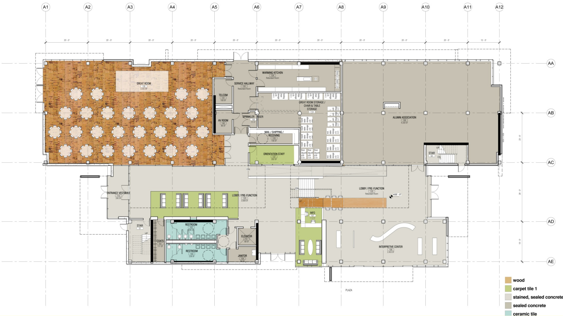
Level One Floor Plan
