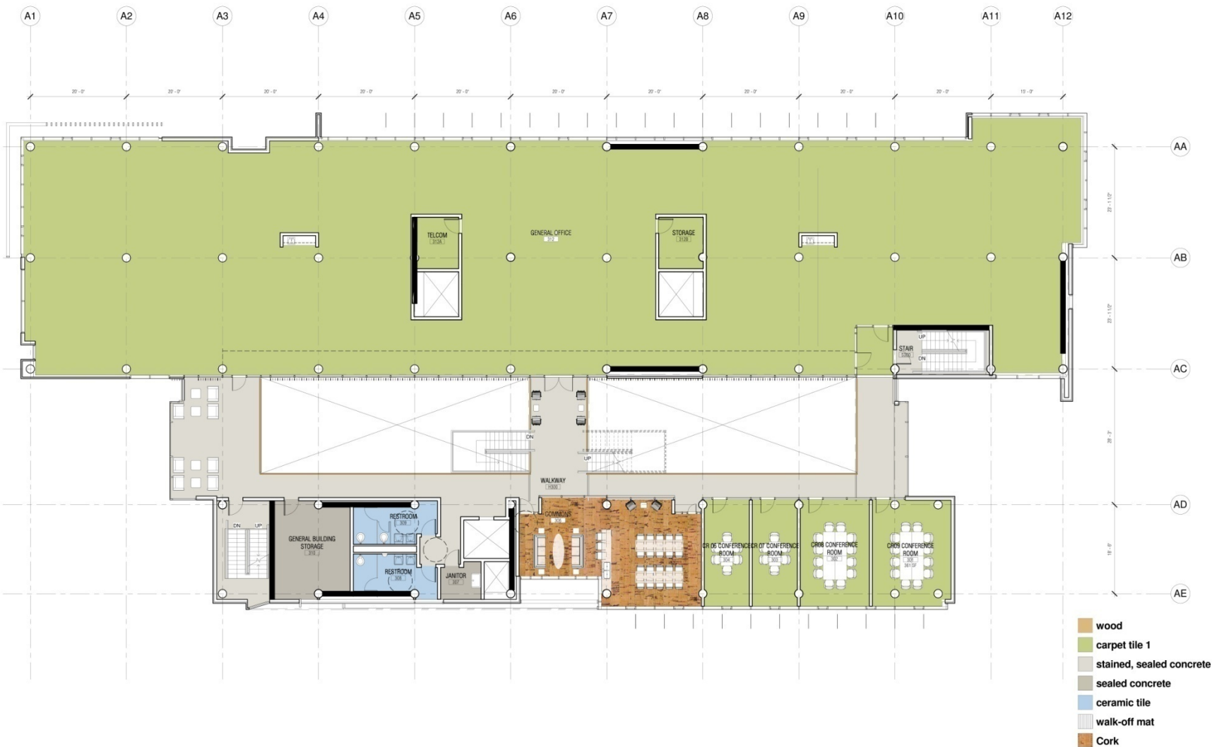
Level Three Floor Plan
